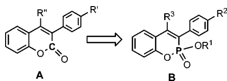
Figure 1. Coumarins ( A ) and the designed phosphacoumarins ( B ) ( R' , R'' , R^1 , R^2 , and R^3 are various substituents).
